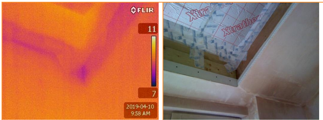
10.02: Thermographic image showing leakage at wood-to-wood joint in corner below rooflight
